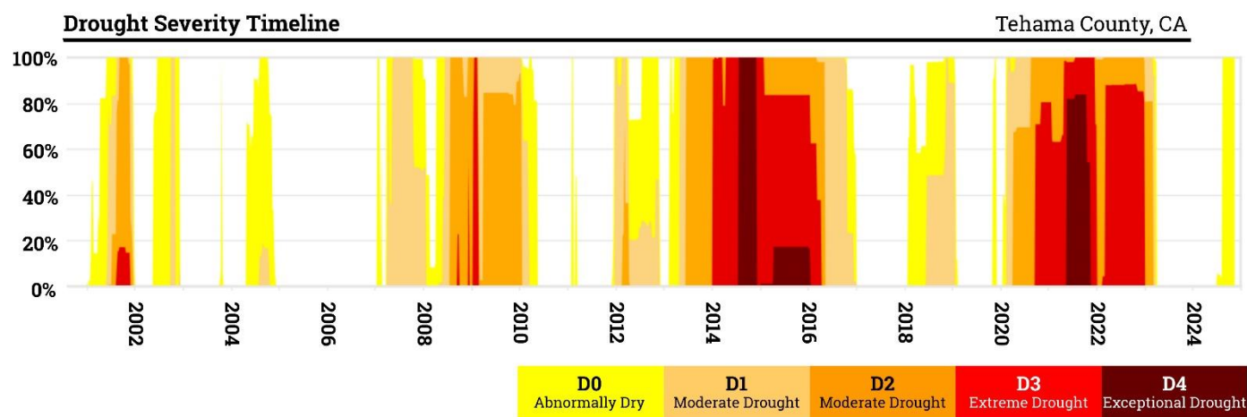
Figure 4-39: Tehama County Drought Severity Timeline 2000-2024
