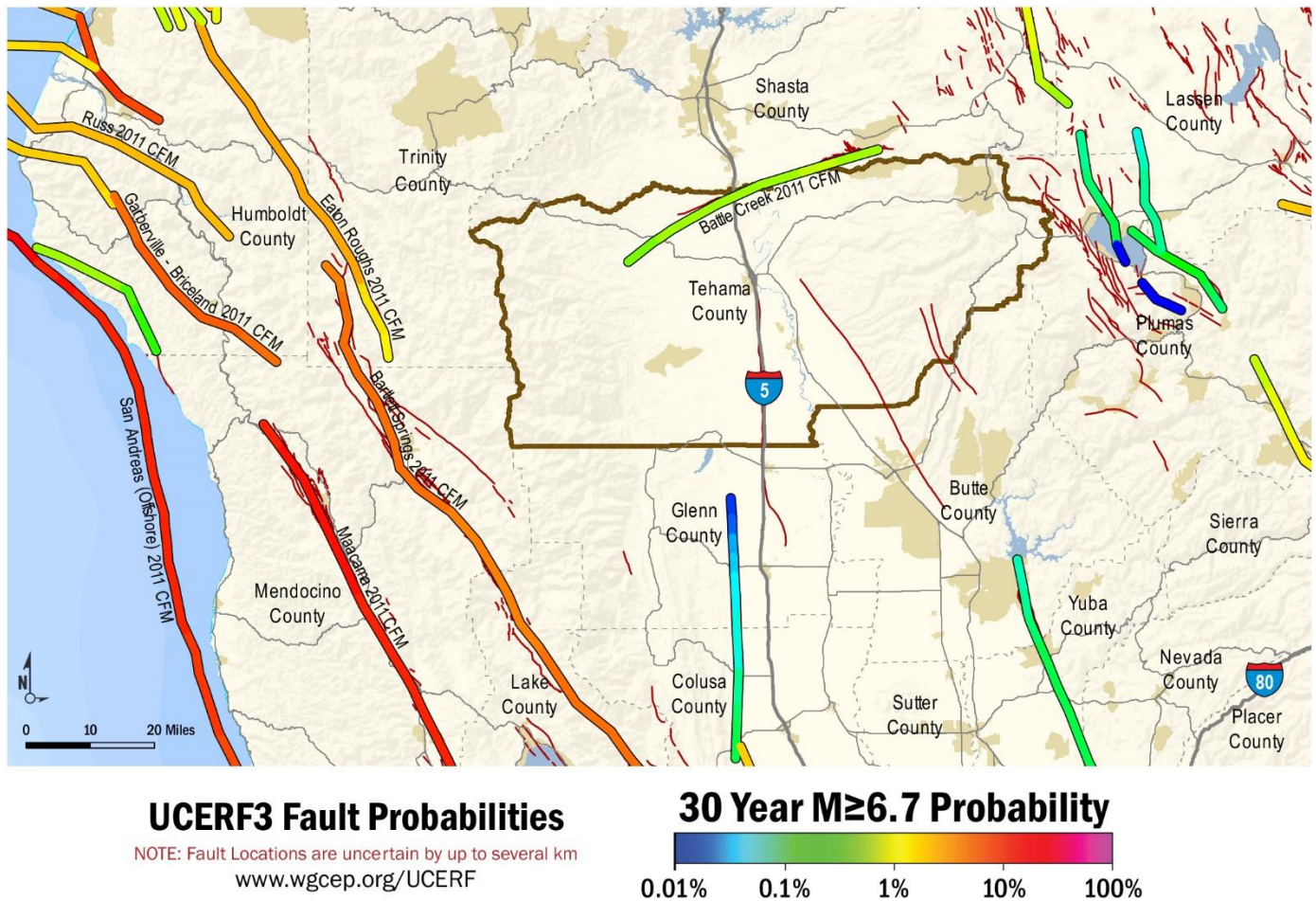
Figure 4-33 Tehama County UCERF3
